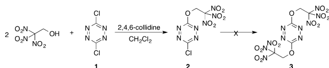
Scheme 1. Nucleophilic reaction of 2,2,2-trinitroethanol with 1 .
